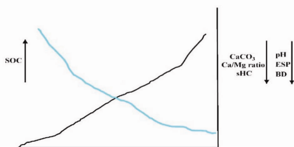
Figure 7. Schematic diagram showing relation between climate (rain-fall), chemical (soil organic carbon, SOC; CaCO 3 ; soil reactions, pH; extractable calcium/magnesium ratio exchangeable sodium percentage (ESP); and physical parameters (bulk density, BD; saturated hydraulic conductivity, sHC) in soils.
