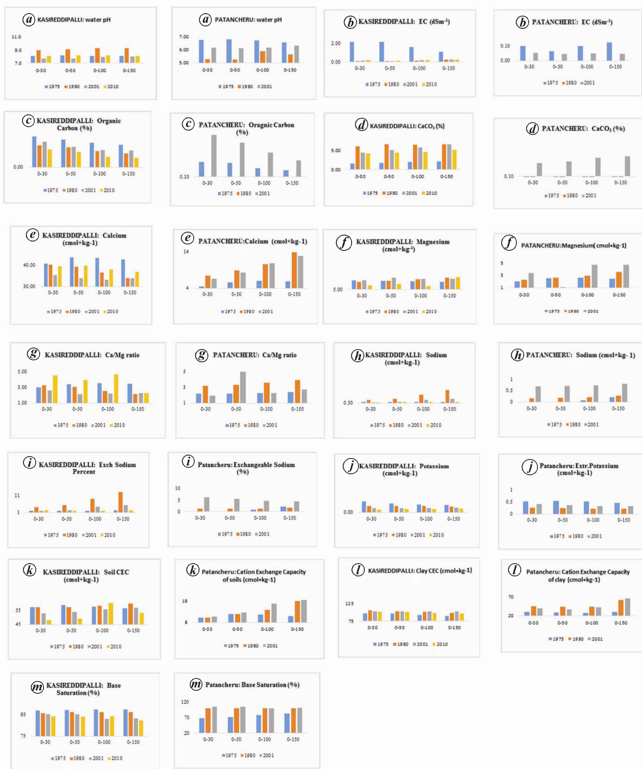
Figure 6. Changes in chemical properties over time in black (Kasireddipalli) and red (Patancheru) soils. a , Water pH; b , electrical conductivity; c , organic carbon; d , \text{CaCO}_3 ; e , extractable calcium; f , extractable magnesium; g , extractable calcium/magnesium ratio; h , extractable sodium; i , exchangeable sodium percentage; j , extractable potassium; k , soil CEC; l , clay CEC; m , base saturation.
