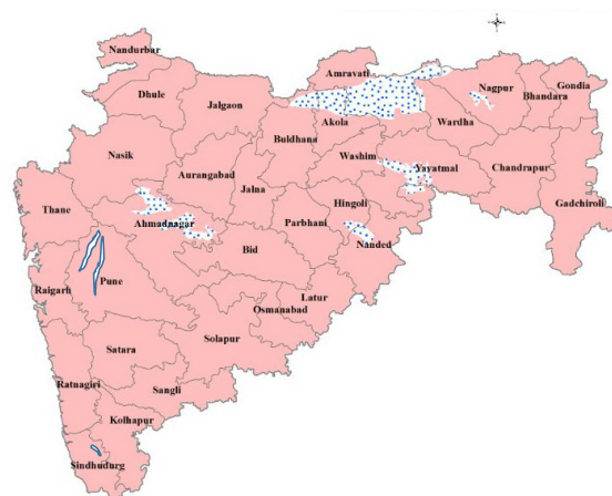
Fig. 31. Distribution of zeolitic soils in Maharashtra.
