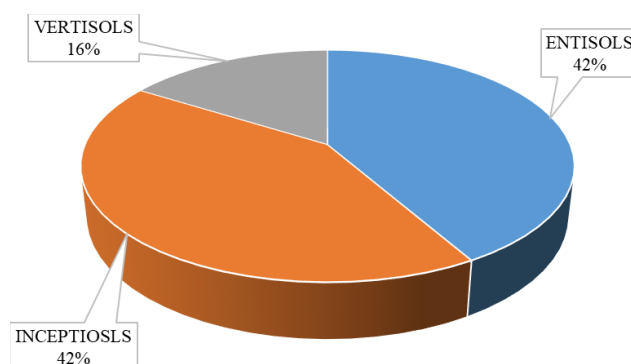
Fig. 13. Soils of Thane and Palghar districts and their distribution.
