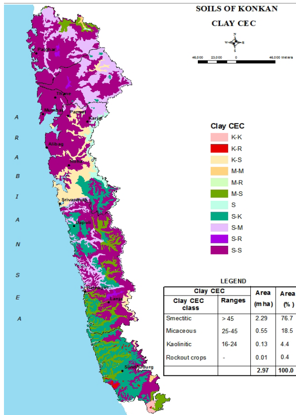
Fig. 14. Soils of Konkan: cation exchange capacity of clay (cmol+kg -1 )
