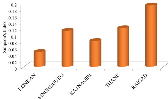
Fig. 22. Simpson's index of dominance in different districts of Konkan region and for the region at the taxonomic level of soil series.
